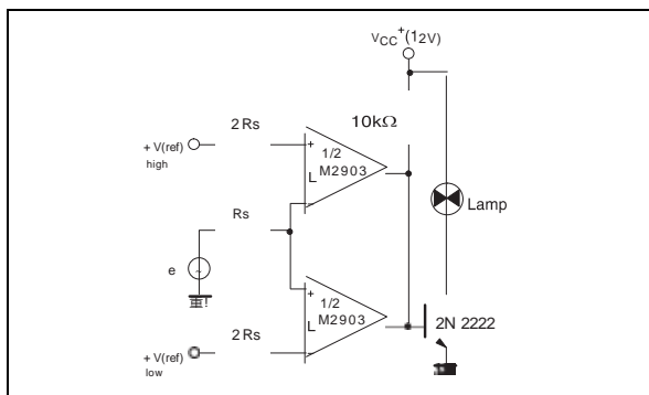
Limit comparator
