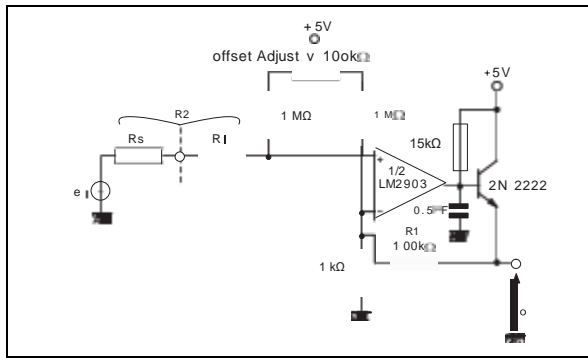
Low frequency op amp with offset adjust
