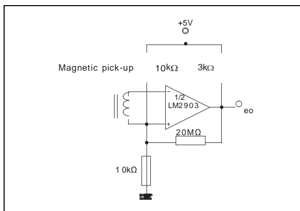
Transducer amplifier
