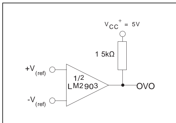
Basic comparator
