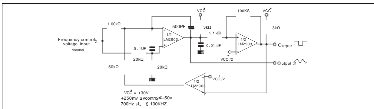
Two-decade high-frequency Vco
