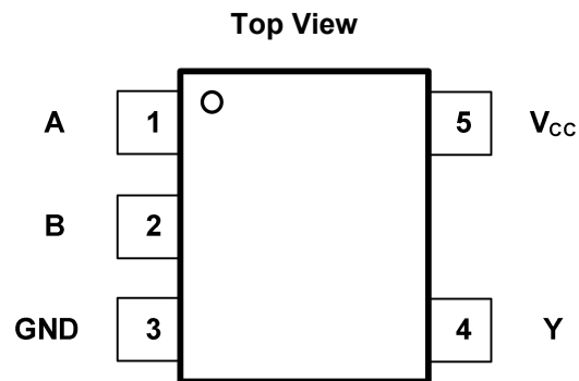
Fig. 5-1. 74LVC1G32: S5 (SOT-23) Package 74LVC1G32: C5 (SC70-5) Package
